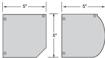
Non-ZIP 127XL angled headbox (side view)
